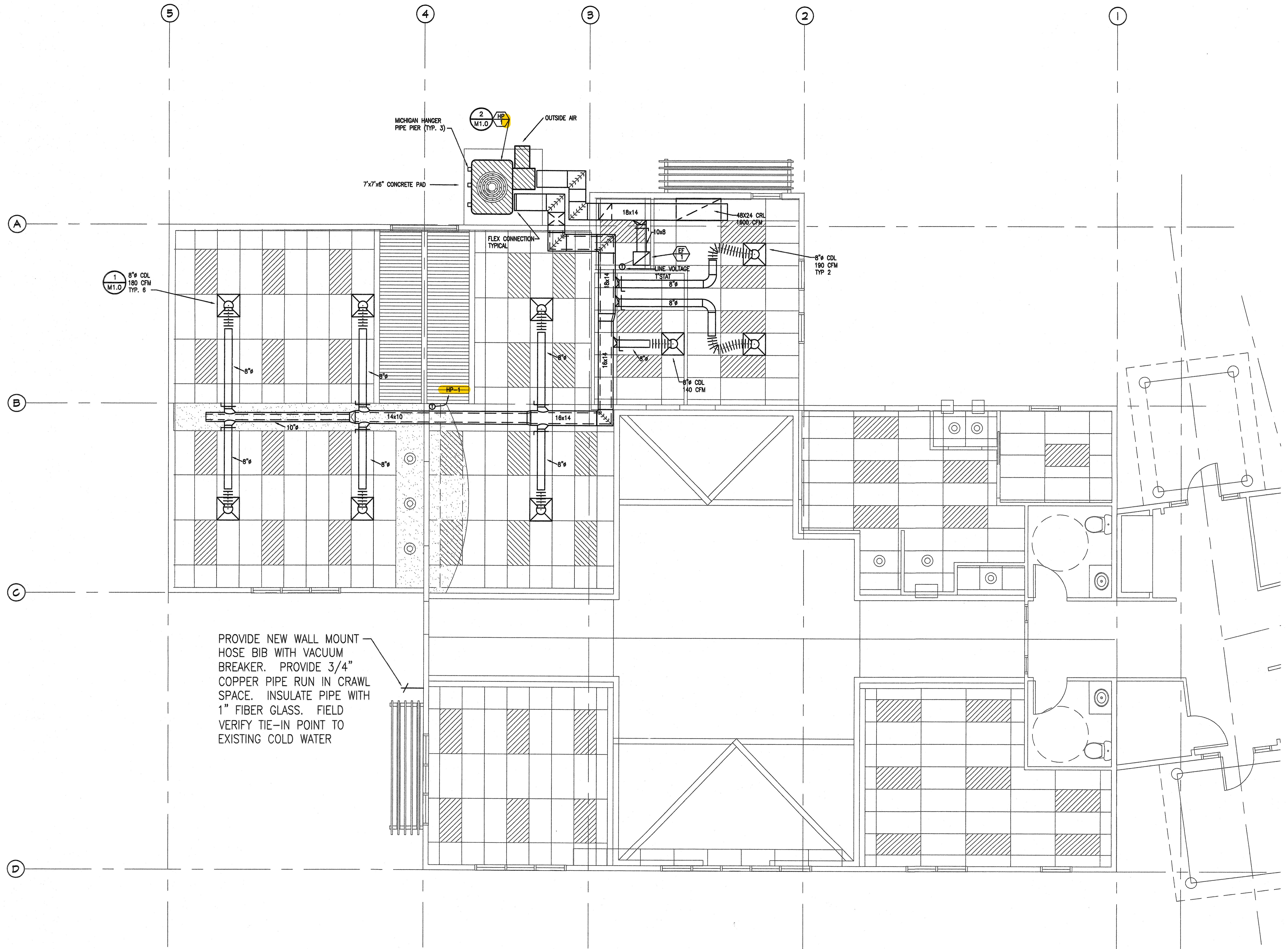
PLAN NORTH HVAC PLAN SCALE: 1/4" = 1'-0"
