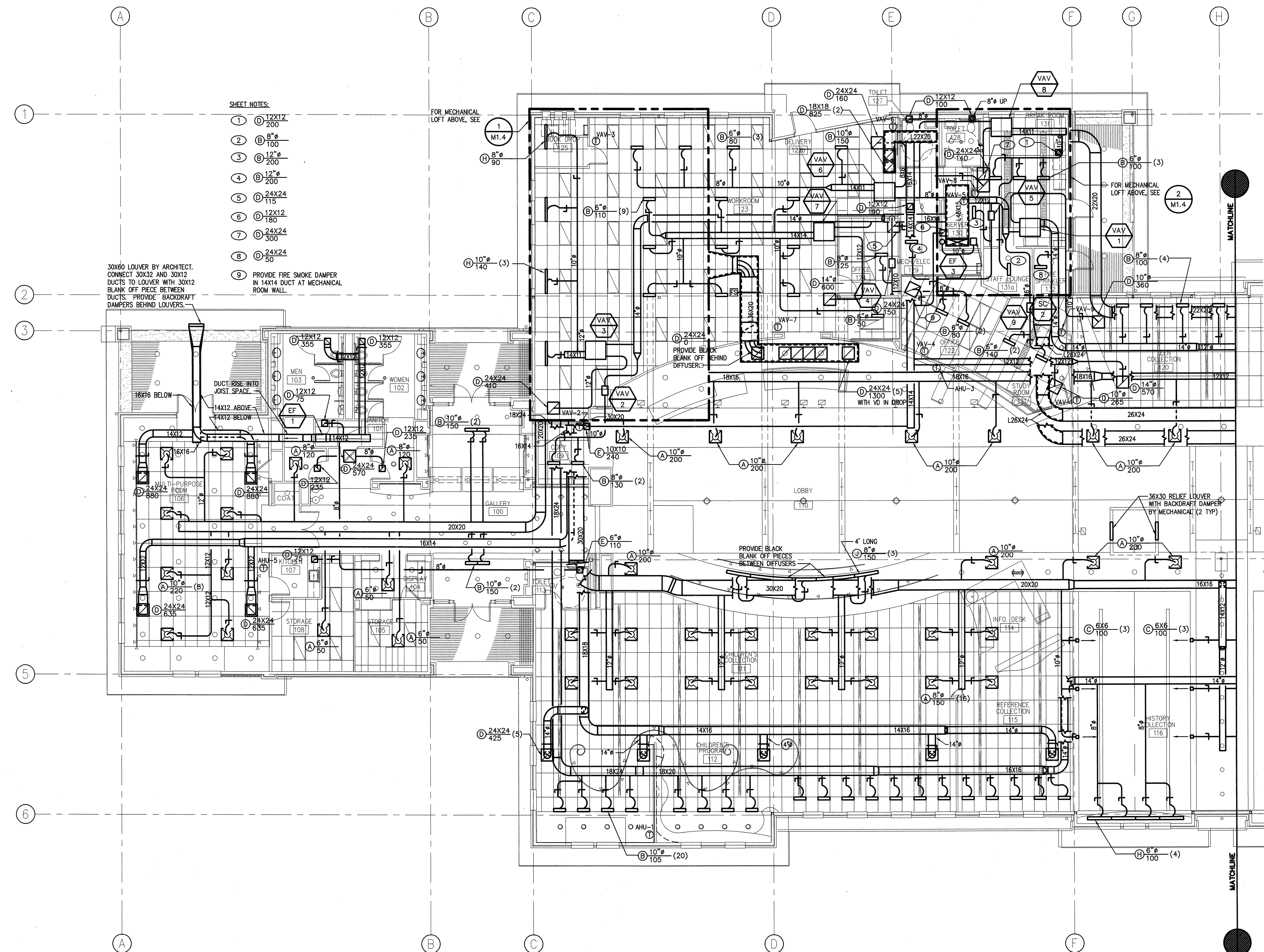
PARTIAL HVAC PLAN SCALE: 1/8"=1'-0" NORTH
